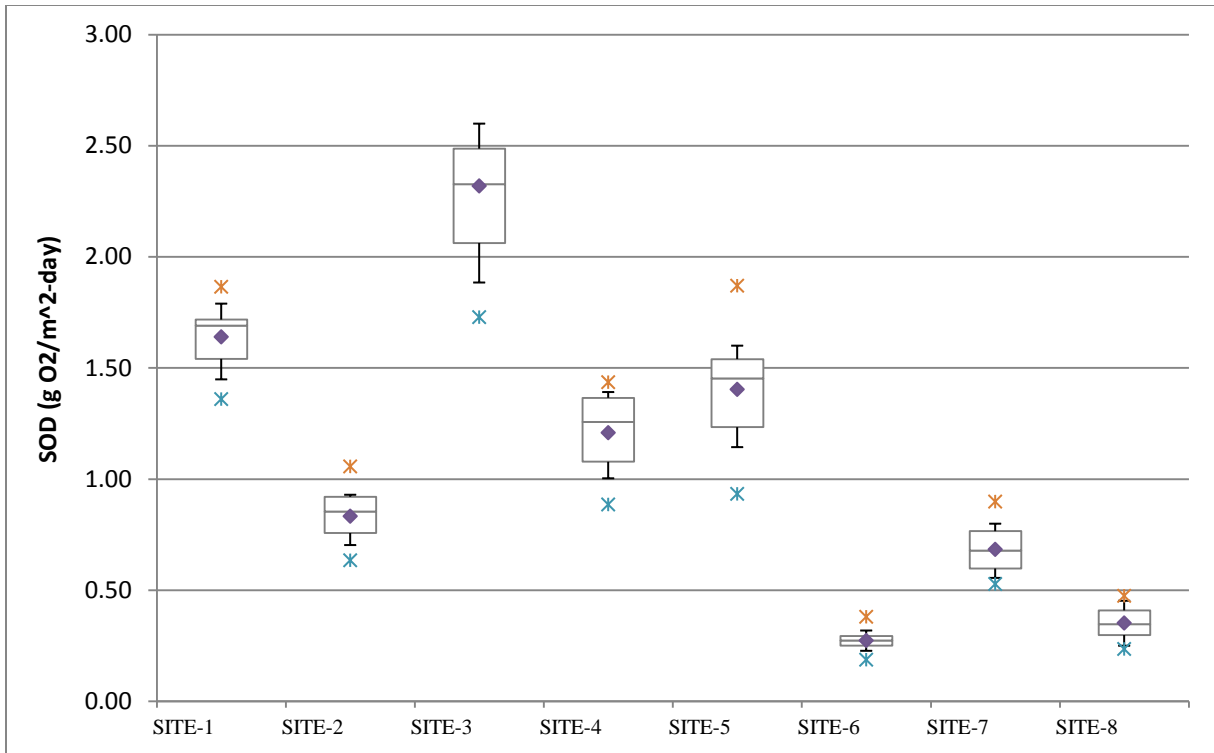
Figure 15. Seasonal stratified summary statistics for simulated SOD from sediment bed
