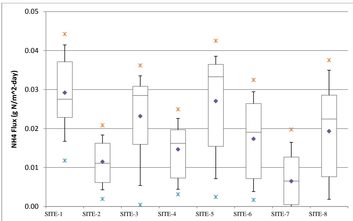
Figure 14. Seasonal stratified summary statistics for simulated NH4 flux from sediment bed
