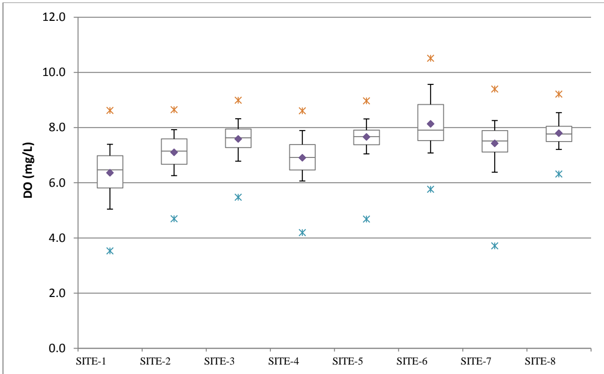
Figure 11. Seasonal stratified summary statistics for simulated DO at surface layer
