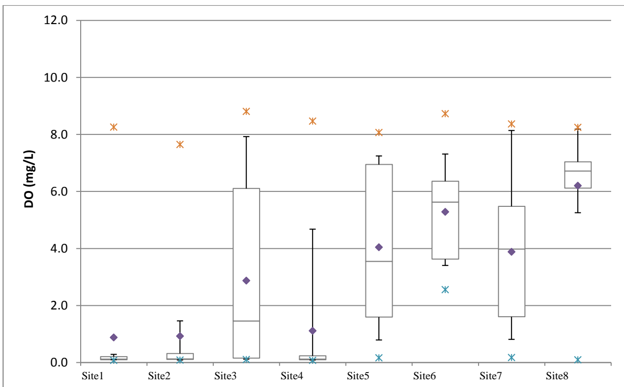
Figure 4. Seasonal stratified summary statistics observed DO at bottom layer
