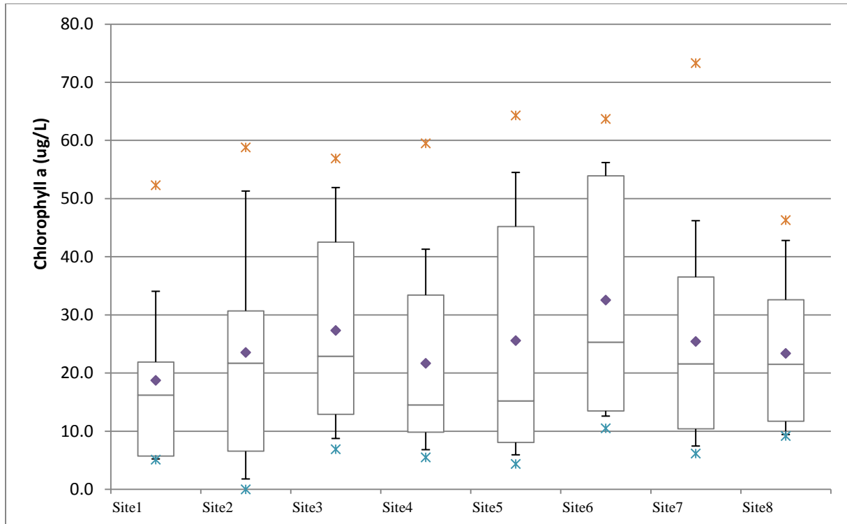
Figure 1. Annual summary statistics for observed chlorophyll a at surface layer
