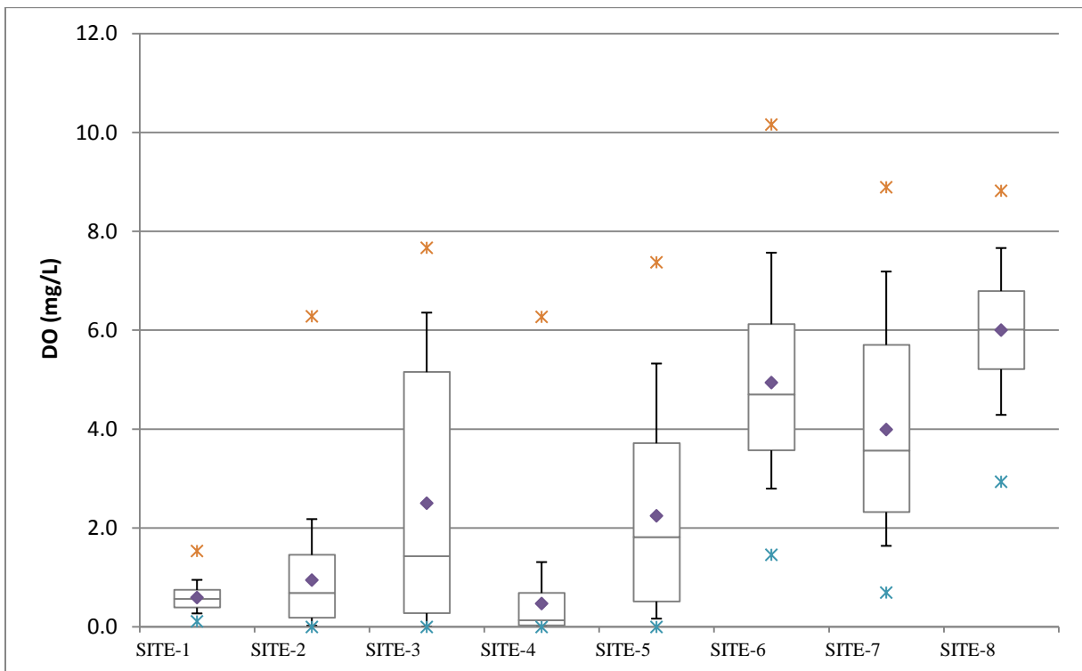
Figure 12. Seasonal stratified summary statistics for simulated seasonal DO at bottom layer
