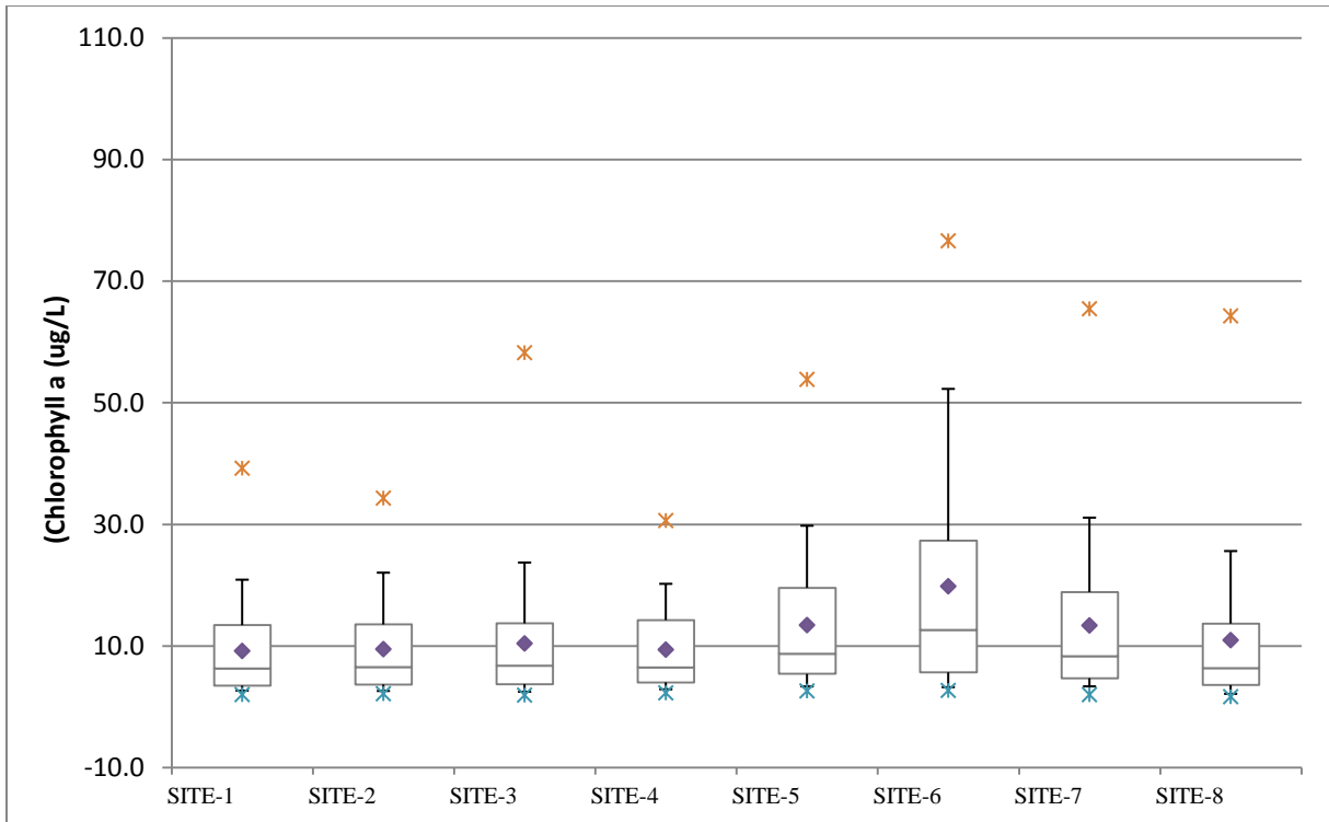
Figure 7. Non-stratified summary statistics for simulated chlorophyll a at surface layer
