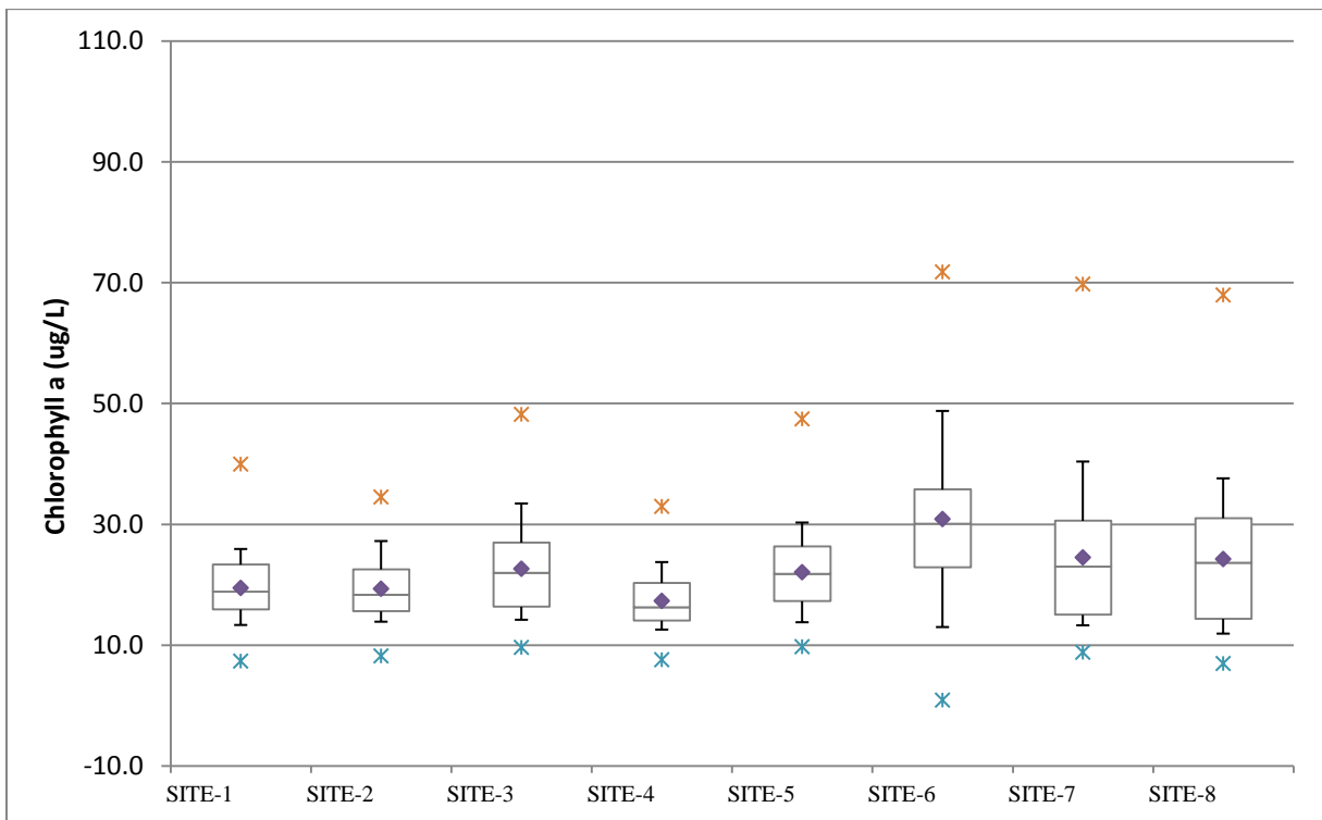
Figure 6. Seasonal stratified summary statistics for chlorophyll a at surface layer
