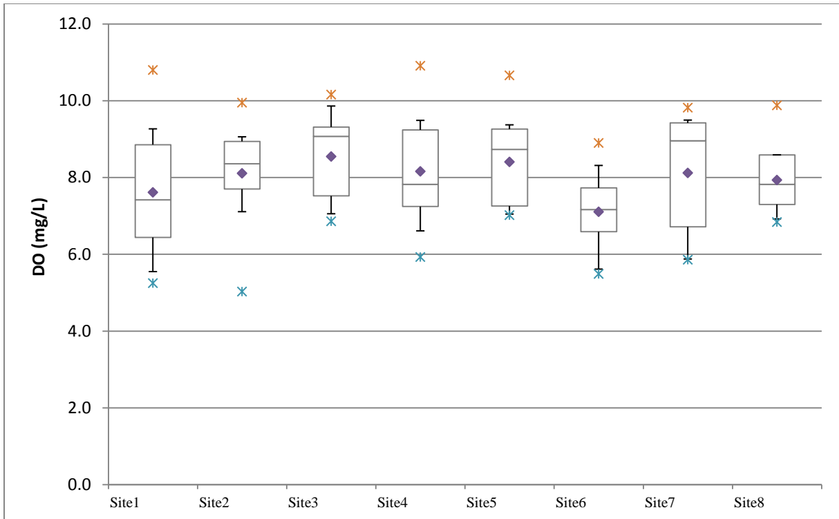
Figure 3. Seasonal stratified summary statistics for observed DO at surface layer
