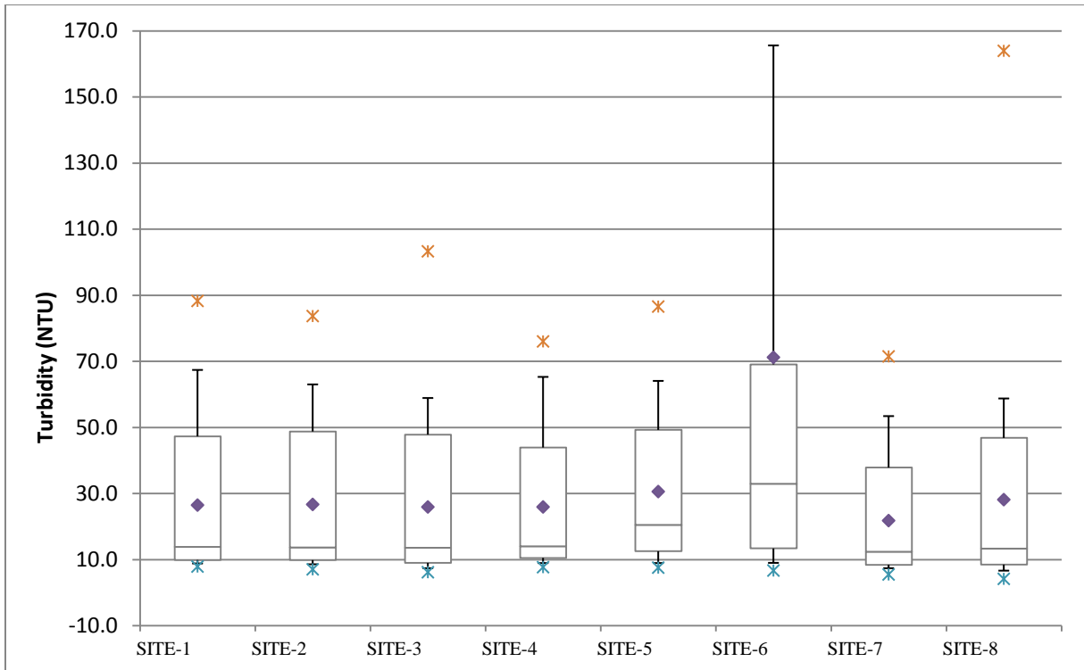
Figure 9. Seasonal stratified summary statistics for simulated turbidity at surface layer
