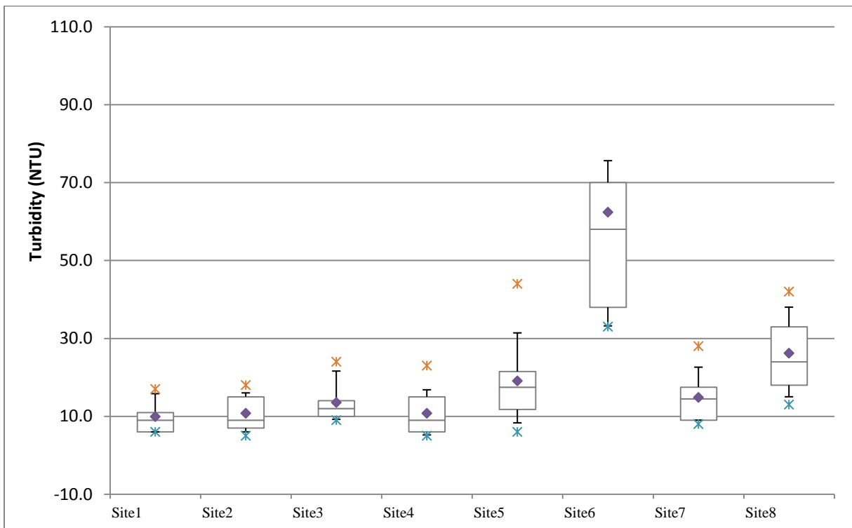
Figure 2. Annual summary statistics for observed turbidity at surface layer
