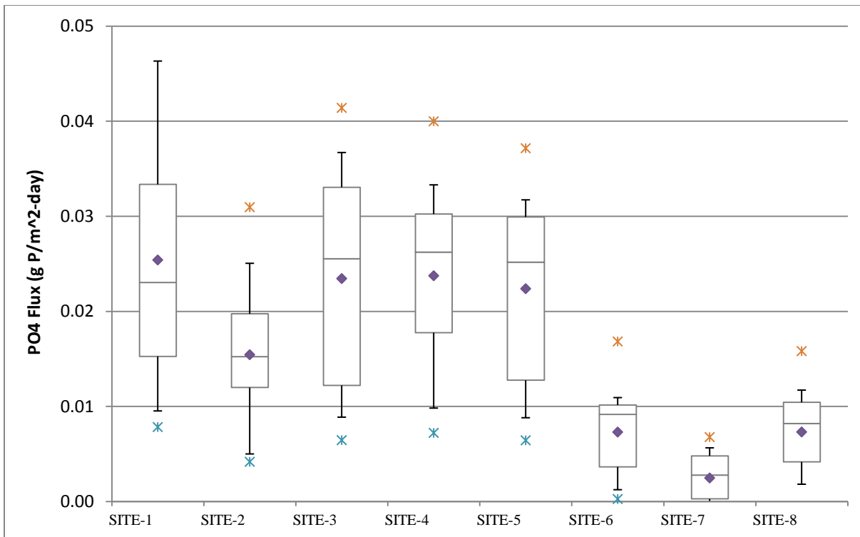
Figure 13. Seasonal stratified summary statistics for simulated PO4 flux from sediment bed
