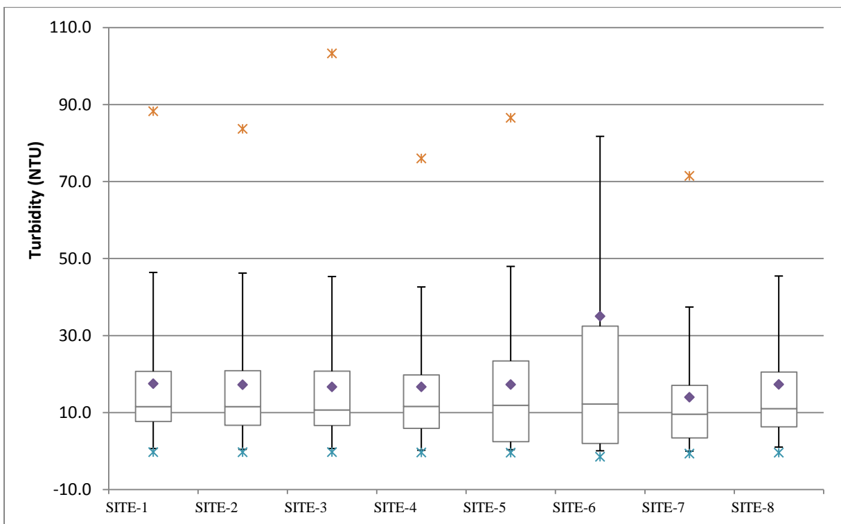
Figure 8. Annual summary statistics for simulated turbidity at surface layer
