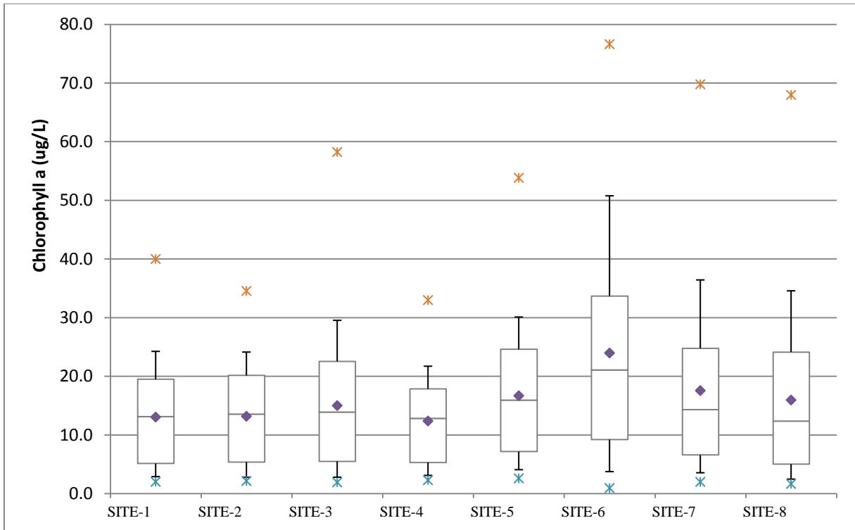
Figure 5. Annual summary statistics for simulated chlorophyll a at surface layer
