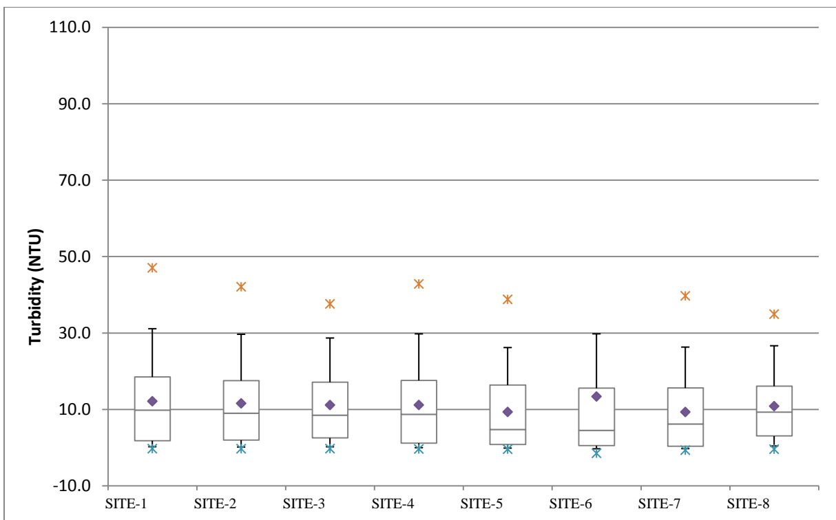
Figure 10. Non-stratified summary statistics for simulated turbidity at surface layer
