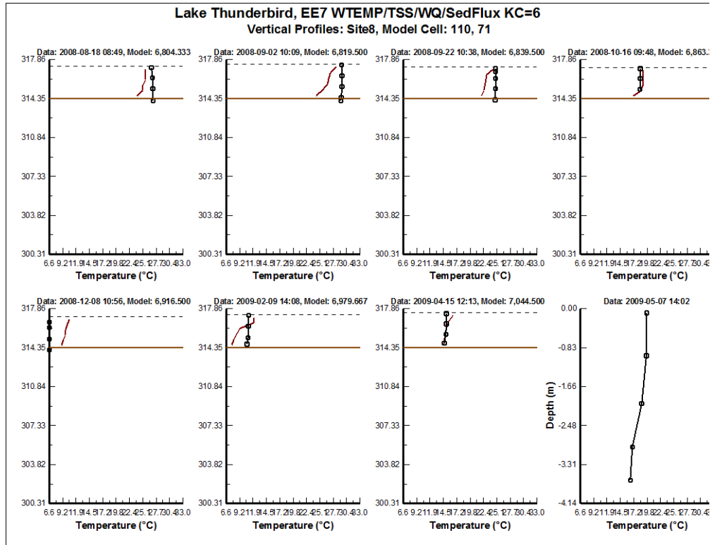
Figure 8. Vertical profile plot of water temperature at Site 8 (continued)
