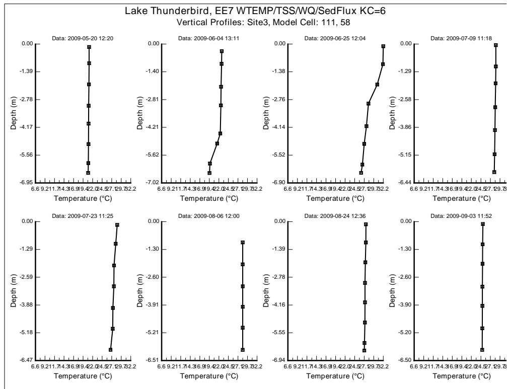
Figure 3. Vertical profile plot of water temperature at Site 3 (continued)
