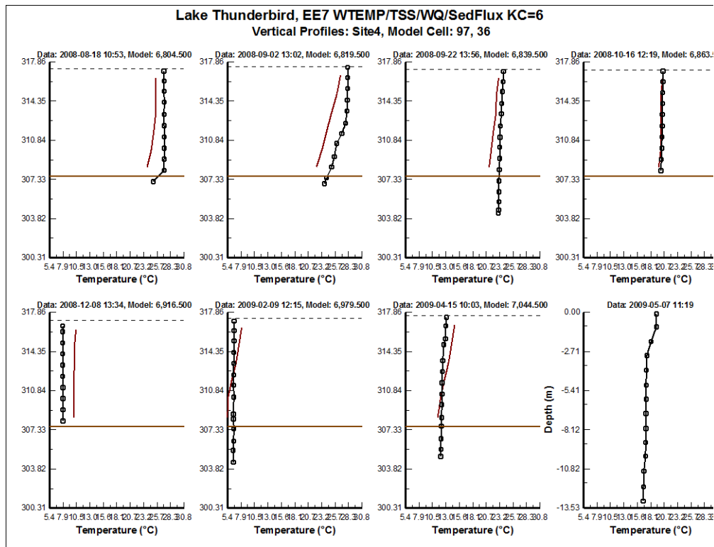
Figure 4. Vertical profile plot of water temperature at Site 4 (continued)
