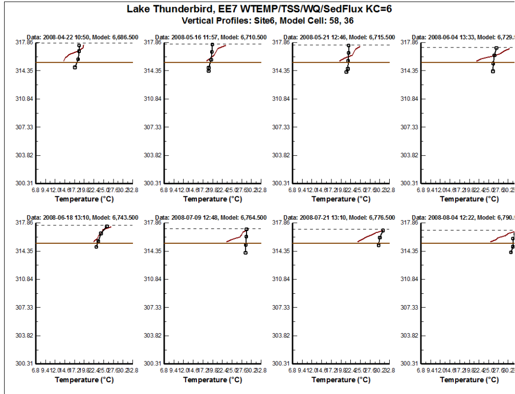
Figure 6. Vertical profile plot of water temperature at Site 6
