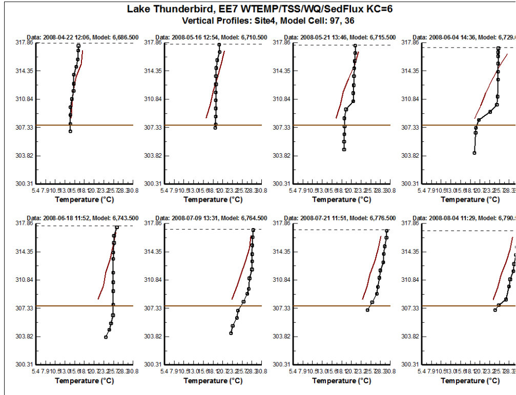
Figure 4. Vertical profile plot of water temperature at Site 4
