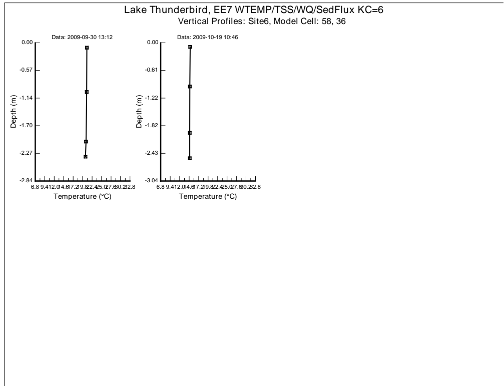
Figure 6. Vertical profile plot of water temperature at Site 6 (continued)
