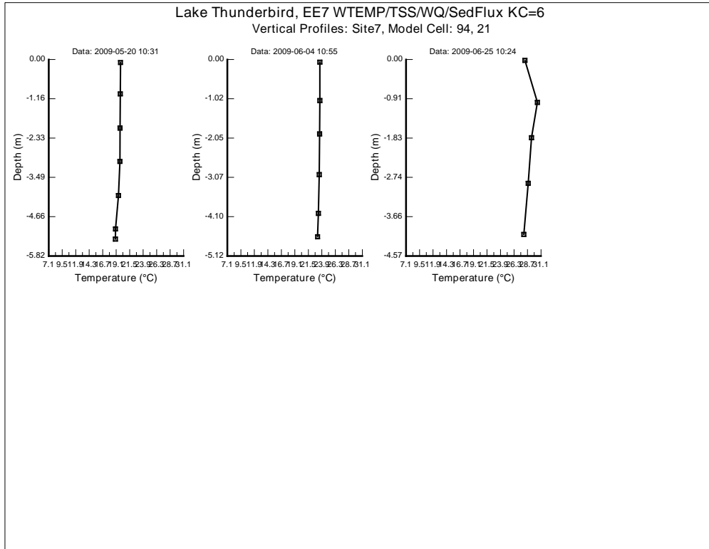
Figure 7. Vertical profile plot of water temperature at Site 7 (continued)
