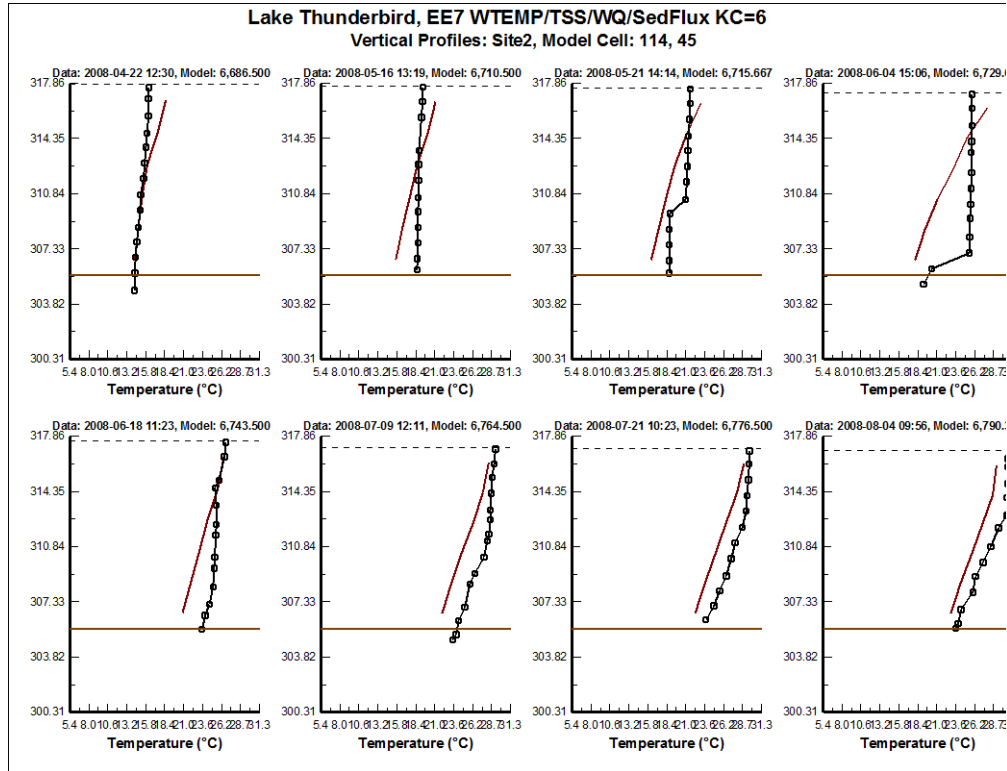
Figure 2. Vertical profile plot of water temperature at Site 2
