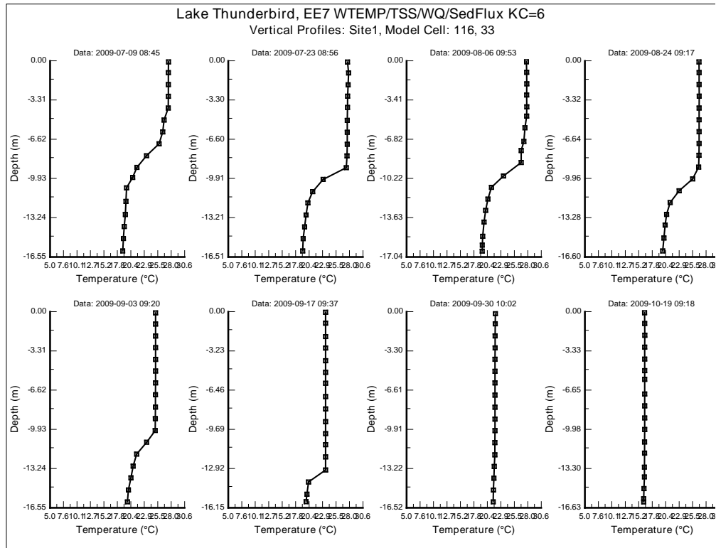
Figure 1. Vertical profile plot of water temperature at Site 1 (continued)
