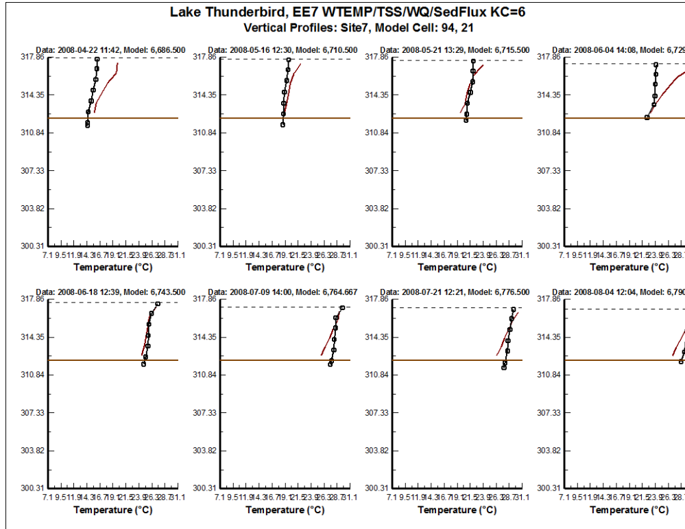
Figure 7. Vertical profile plot of water temperature at Site 7
