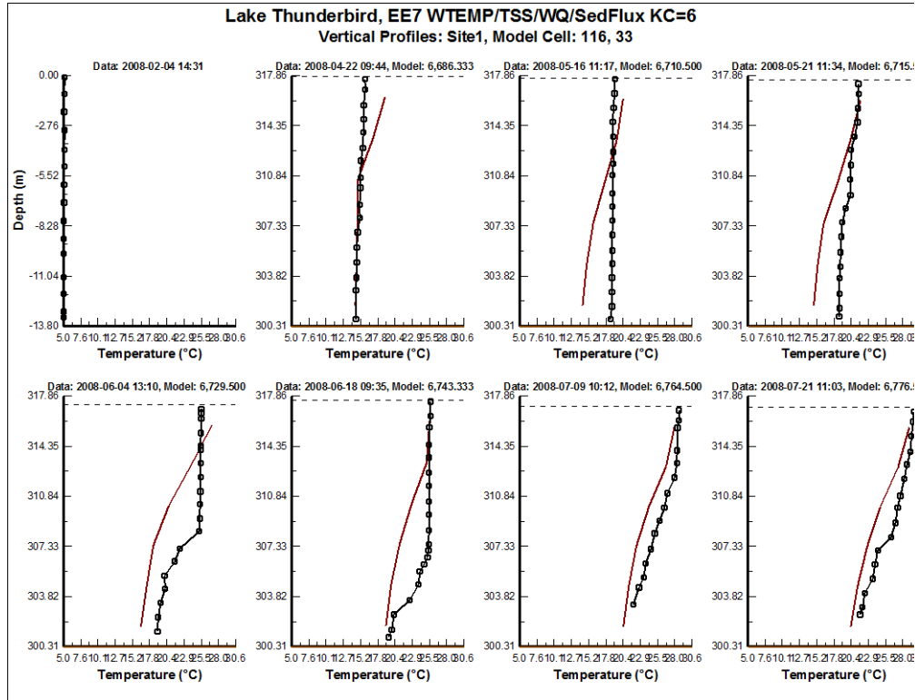
Figure 1. Vertical profile plot of water temperature at Site 1
