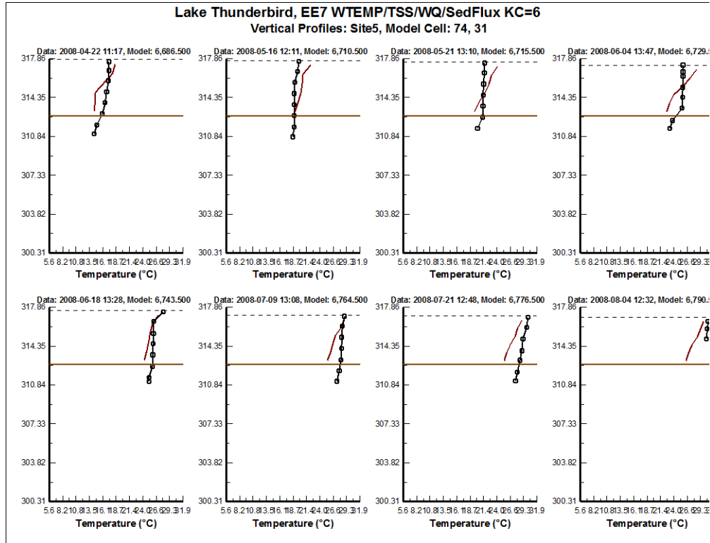
Figure 5. Vertical profile plot of water temperature at Site 5
