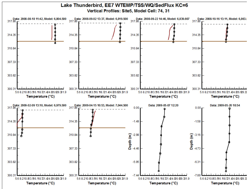
Figure 5. Vertical profile plot of water temperature at Site 5 (continued)
