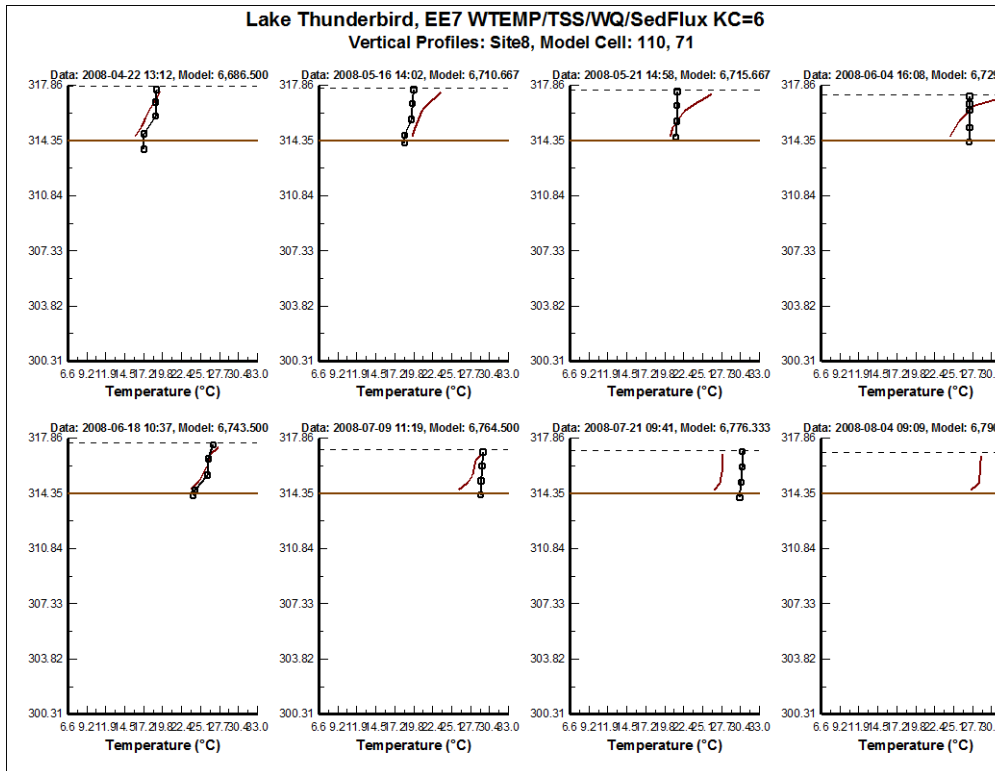
Figure 8. Vertical profile plot of water temperature at Site 8
