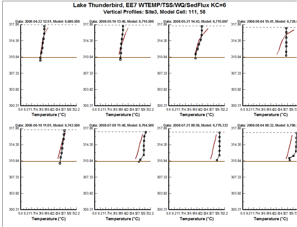
Figure 3. Vertical profile plot of water temperature at Site 3
