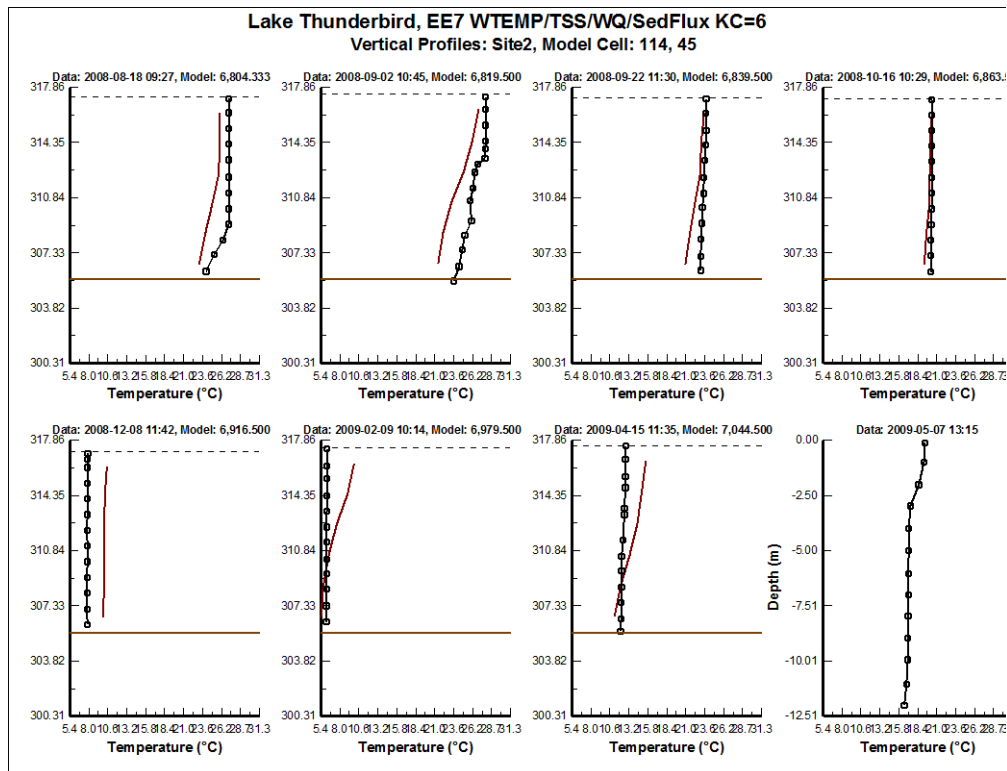
Figure 2. Vertical profile plot of water temperature at Site 2 (continued)
