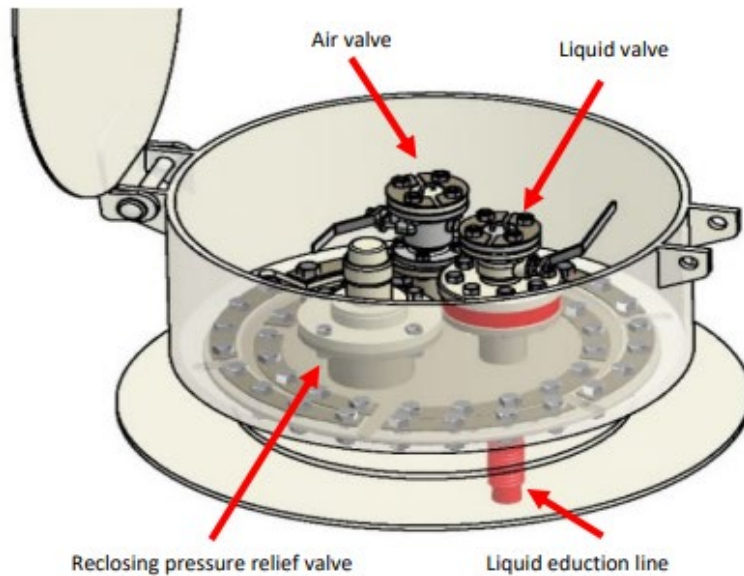
Typical 20-inch HCl Manway
