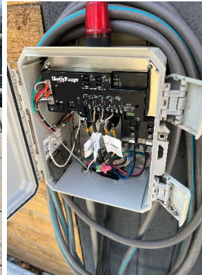
Photo Series #2. Barnacle Bills Marina & Resort September 4, 2024 Holding Tanks, Pump-out systems, shut-off valves, piping under the marina connecting to the aerobic system on land.
