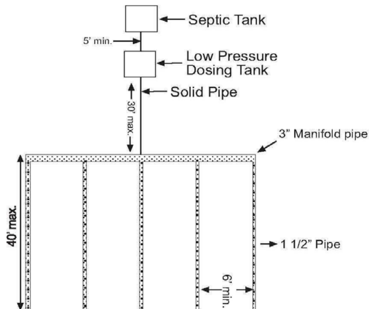
Figure 3. Low Pressure Dosing
