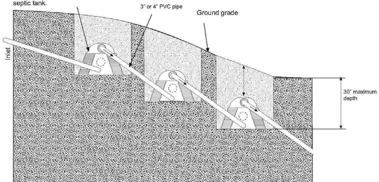
Figure 2. Retention Systems
