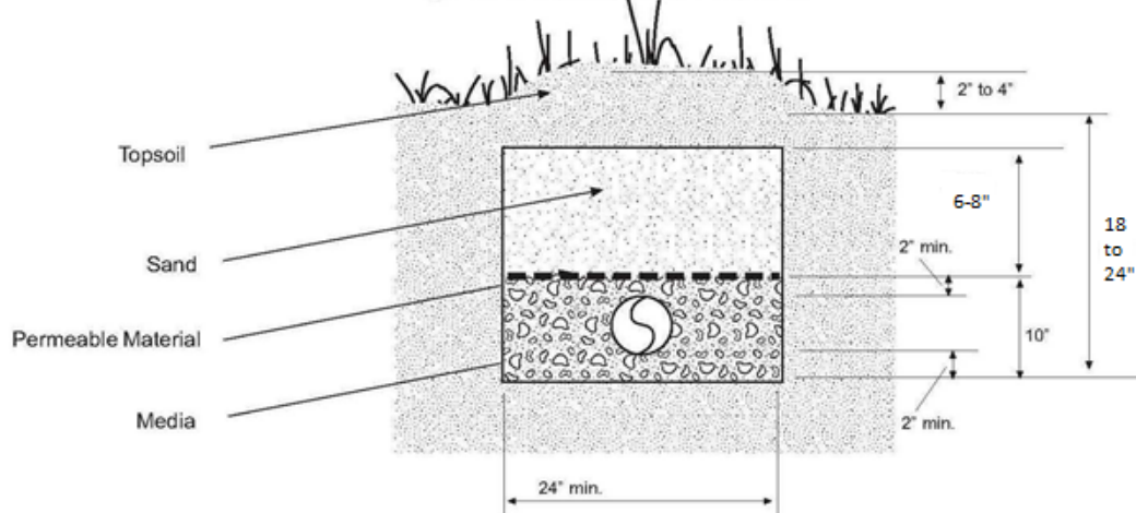
Figure 3. Cross-Section of Low Pressure Dosing
