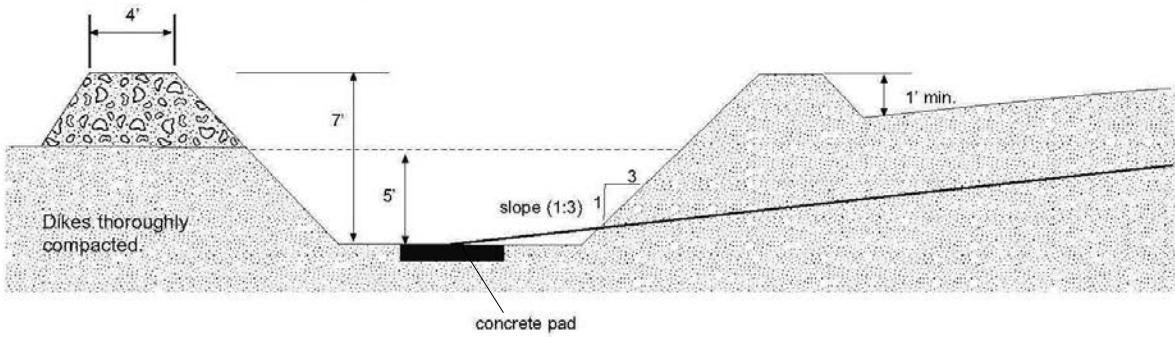
Figure 2. Lagoon Detail
