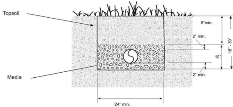
Figure 2. Cross-Section of ET/A Trench
