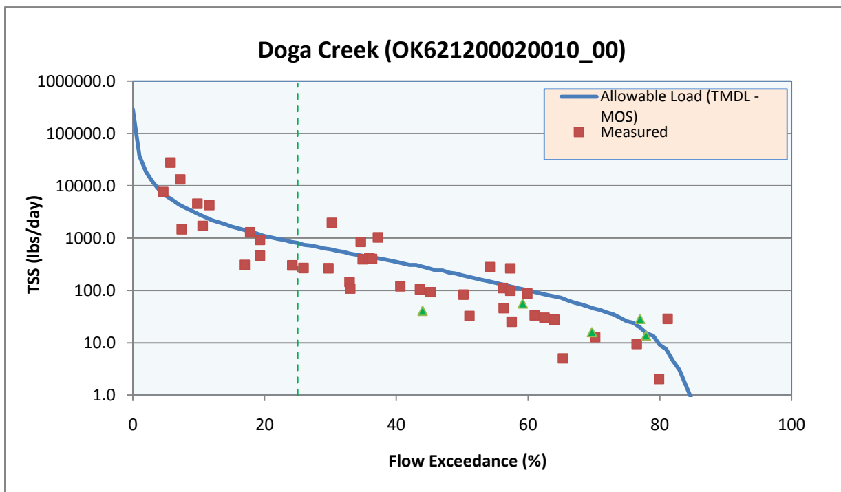
Figure 5-3 Load Duration Curve for Total Suspended Solids in Doga Creek (OK621200020020_00)
