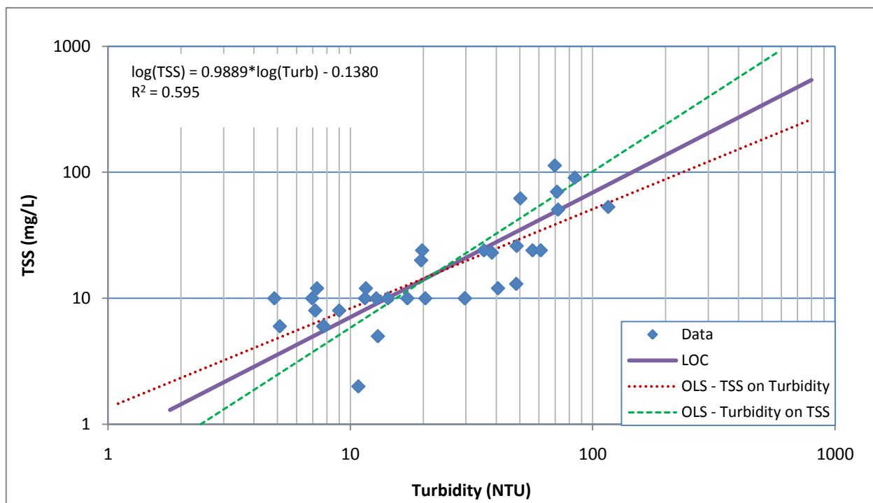
Figure 4-3 Linear Regression for TSS-Turbidity for Doga Creek (OK621200020020_00)
