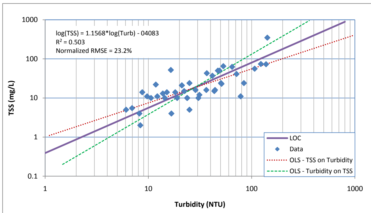
Figure 4-2 Linear Regression for TSS-Turbidity for Gray Horse Creek (OK621200010400_00)
