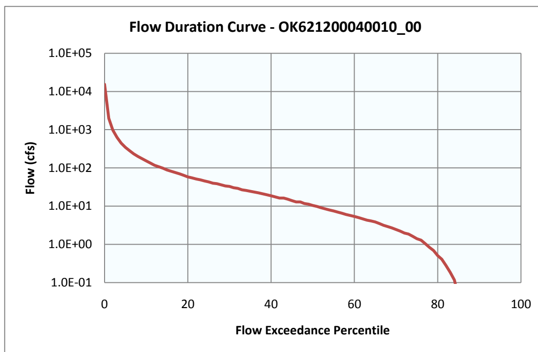
Figure 4-4 Flow Duration Curve for Salt Creek (OK621200040010_00)
