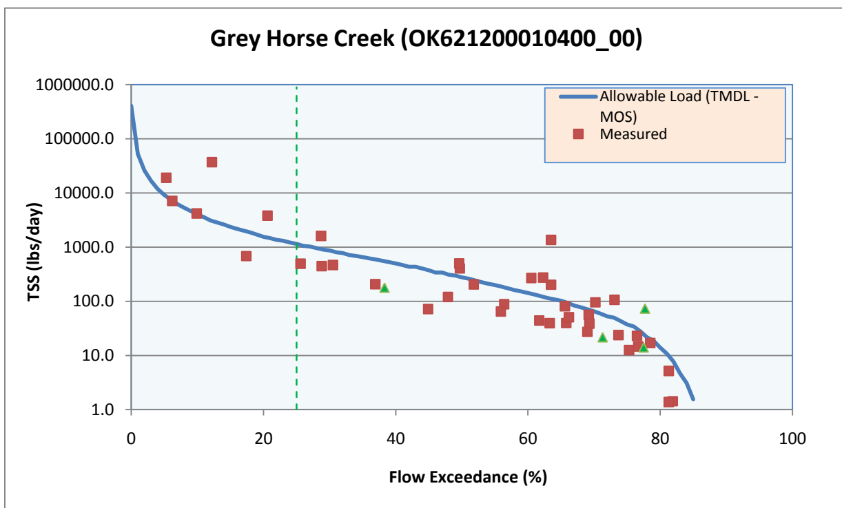
Figure 5-2 Load Duration Curve for Total Suspended Solids in Gray Horse Creek (OK621200010400_00)
