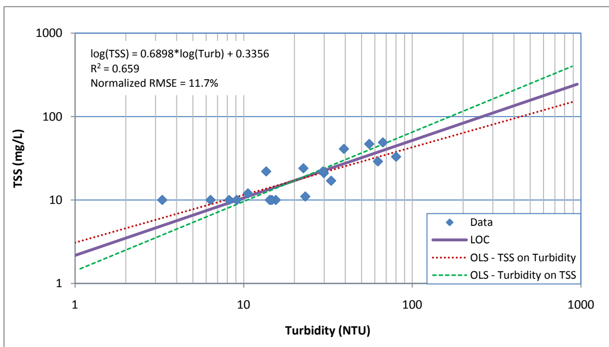
Figure 4-1 Linear Regression for TSS-Turbidity for Salt Creek (OK621200040010_00)
