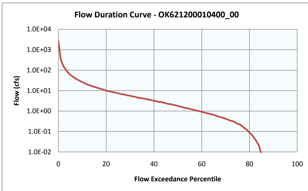
Figure 4-5 Flow Duration Curve for Gray Horse Creek (OK621200010400_00)
