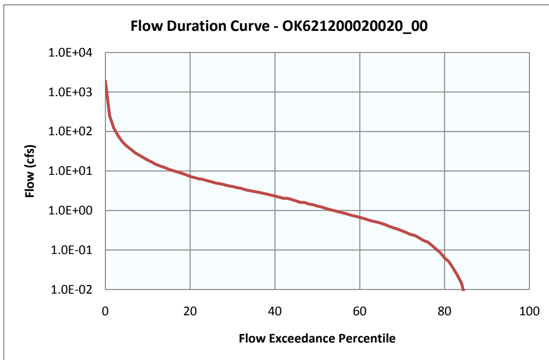
Figure 4-6 Flow Duration Curve for Doga Creek (OK621200020020_00)
