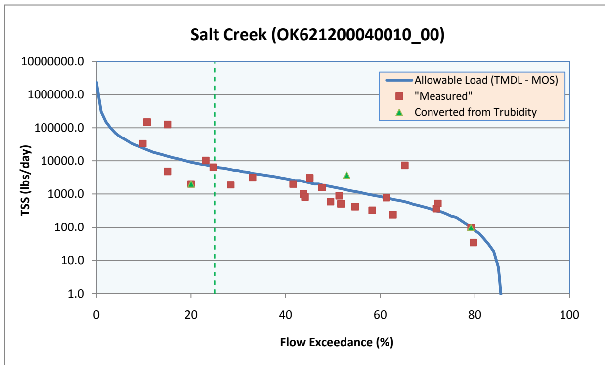
Figure 5-1 Load Duration Curve for Total Suspended Solids in Salt Creek (OK621200040010_00)
