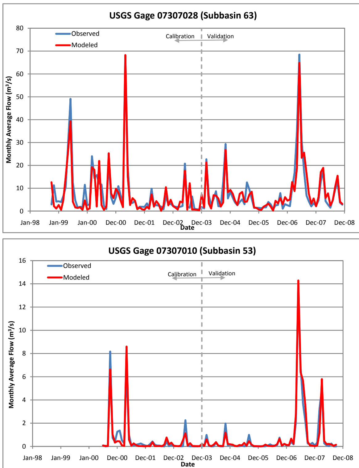
Figure 3-4 Observed and SWAT Modeled Average Monthly Flows
