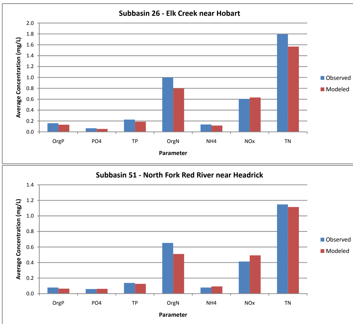
Figure 3-5 Observed and SWAT Modeled Nutrient Concentrations
