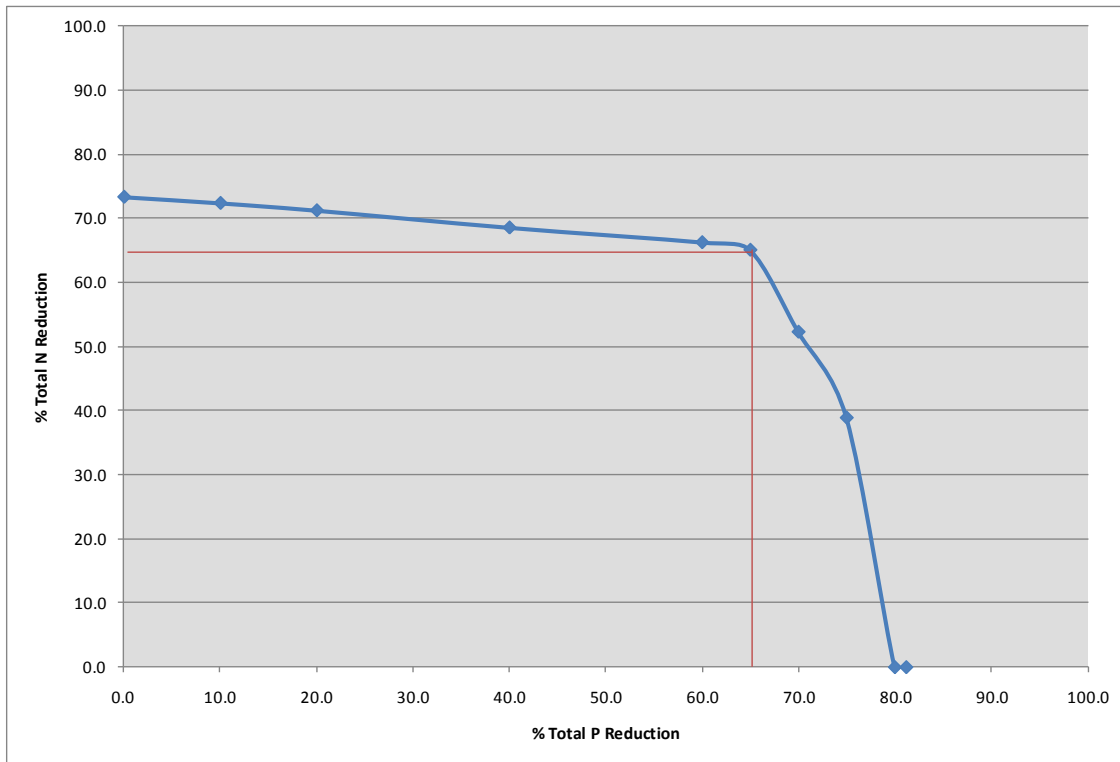
Figure 4-2 Total N and Total P Reduction Combinations Resulting in 10 µg/L Chlorophyll- a - Tom Steed Lake
