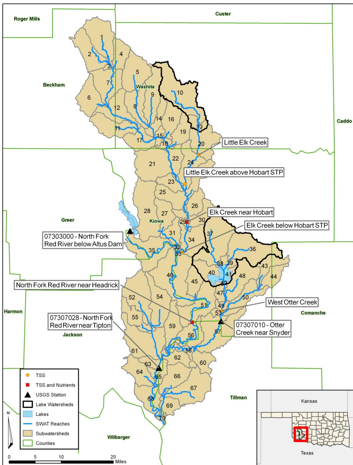
Figure 3-3 Subwatersheds Simulated in the SWAT Watershed Model
