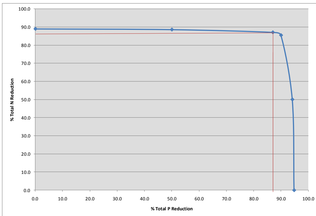
Figure 4-1 Total N and Total P Combinations Resulting in 10 µg/L Chlorophyll- a - Rocky Lake
